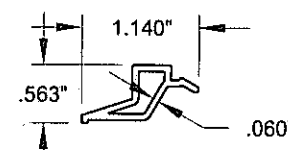
27 7/8" BEVELED BEAD #20024, Rigid PVC
