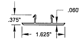
18 1" MULLION CAP #20009, Rigid PVC
