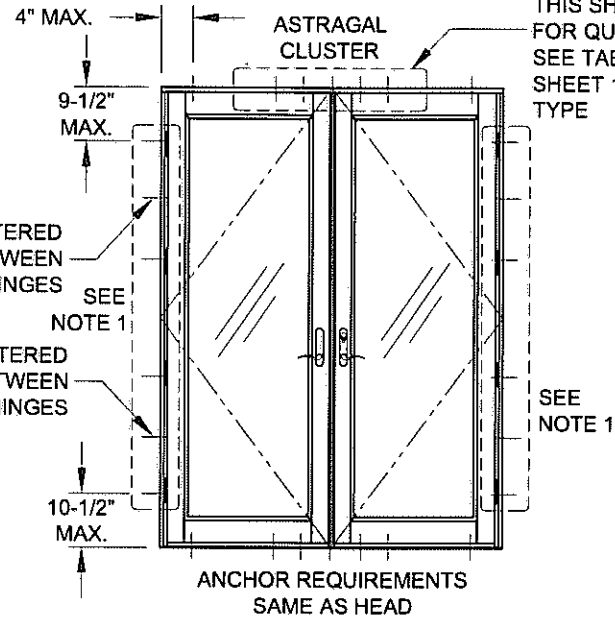
XX, (USING ASTRAGAL)
