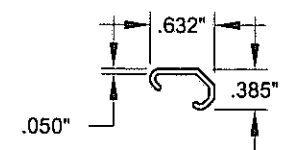
20 SINGLE DOOR ASTRAGAL COVER #20012, Rigid PVC
