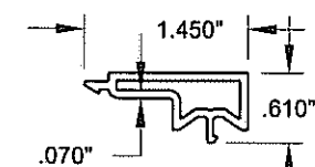
16 FRAME SCREW COVER #20007, Rigid PVC
