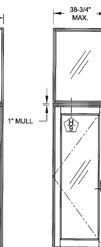
O/X WITH HORIZONTAL MULLION (NARROW STILES AND NARROW RAILS SHOWN ON SIDELITE & TRANSOM)
