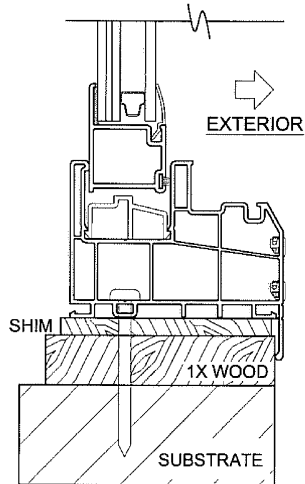
FLANGE FRAME, SILL INSTALLATION (USING 1X BUCKSTRIP)
