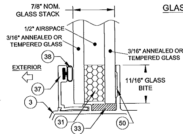
GLASS TYPES 9 & 10
