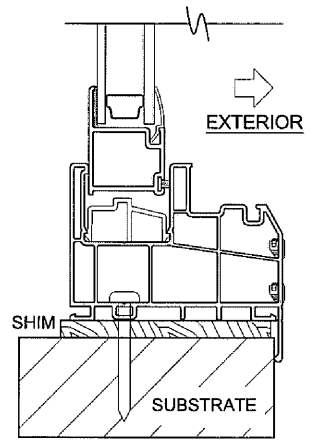
FLANGE FRAME, SILL INSTALLATION (DIRECTLY TO SUBSTRATE)
