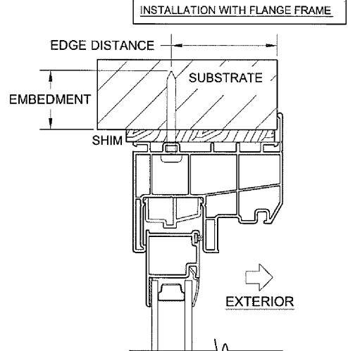
FLANGE FRAME, HEAD INSTALLATION (DIRECTLY TO SUBSTRATE)
