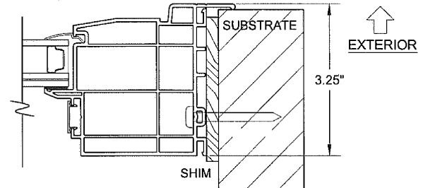
FLANGE FRAME, JAMB INSTALLATION (DIRECTLY TO SUBSTRATE)
