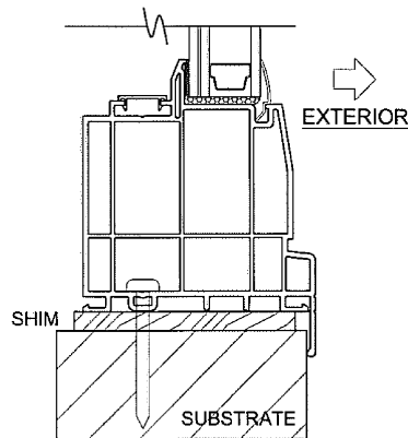
FLANGE FRAME, SILL INSTALLATION (DIRECTLY TO SUBSTRATE)
