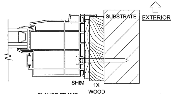
FLANGE FRAME, JAMB INSTALLATION (USING 1X BUCKSTRIP)
