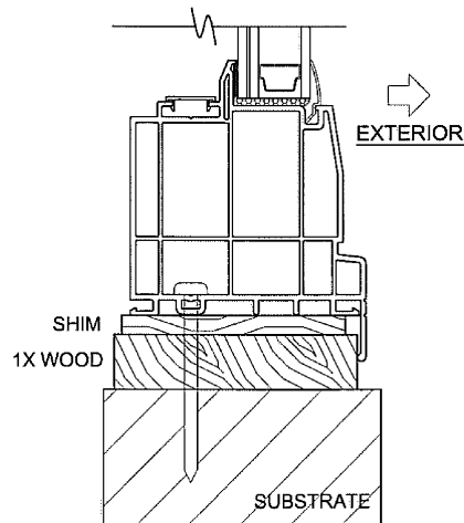
FLANGE FRAME, SILL INSTALLATION (USING 1X BUCKSTRIP)
