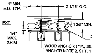
DETAIL B, 2-TRACK FRAME HEAD WOOD INSTALLATION
