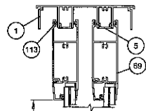
97 7/8" MAX. DLO TYP. DETAIL 'I'
