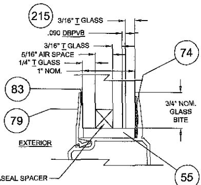
1" LAMINATED I.G. TYPES G8A
