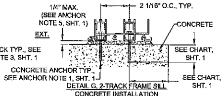
DETAIL G, 2-TRACK FRAME SILL CONCRETE INSTALLATION
