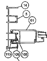
AT MIDSPAN DETAIL 'K' (FIXED PANEL)
