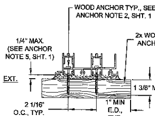
DETAIL C, 2-TRACK FRAME SILL WOOD INSTALLATION
