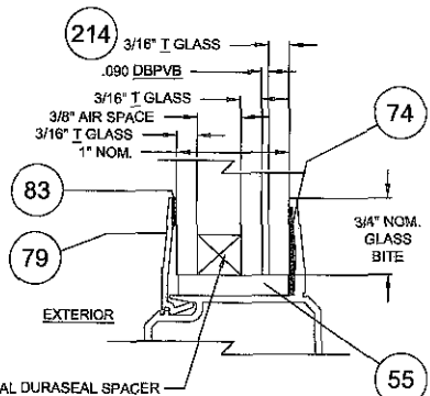
1" LAMINATED I.G. TYPES G8
