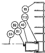
DETAIL 'P' SCREEN AT JAMB
