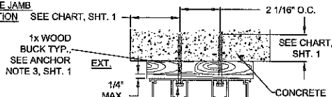
2-TRACK ASTRAGAL / INTERLOCK ANCHOR CLUSTER - C7
