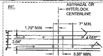
2-TRACK ASTRAGAL / INTERLOCK 8 ANCHOR CLUSTER
