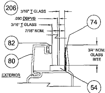
7/16" LAMINATED GLASS TYPES G7
