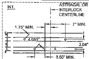
2-TRACK ASTRAGAL / INTERLOCK 8 ANCHOR CLUSTER
