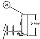
LOW BOX SILL RISER
