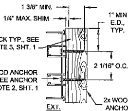
DETAIL E, 2-TRACK FRAME JAMB WOOD INSTALLATION
