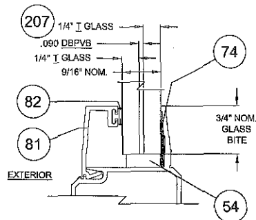
9/16" LAMINATED GLASS TYPES G7A
