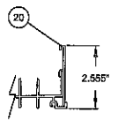
LOW FLAT SILL RISER
