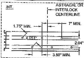
2-TRACK ASTRAGAL / INTERLOCK 6 ANCHOR CLUSTER
