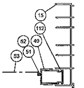
DETAIL 'P' SCREEN AT JAMB
