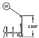
LOW FLAT SILL RISER
