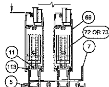
DETAIL 'H'
