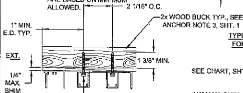
DETAIL A, 2-TRACK W/ SCREEN FRAME HEAD WOOD INSTALLATION
