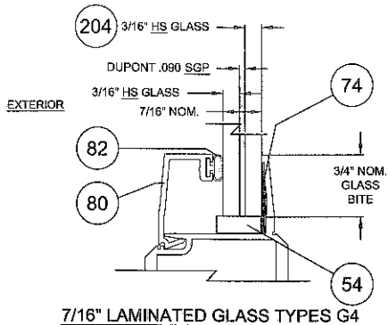
7/16" LAMINATED GLASS TYPES G4
