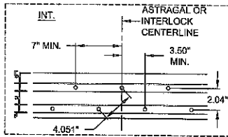
2-TRACK ASTRAGAL / INTERLOCK ANCHOR CLUSTER - C7
