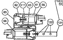
ALL REINFORCED INTERLOCK DETAIL 'J'
