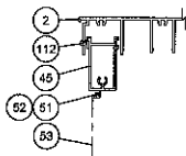
DETAIL 'N' SCREEN AT HEAD
