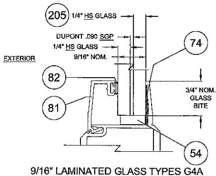
9/16" LAMINATED GLASS TYPES G4A
