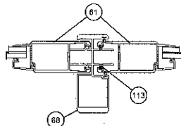
ASTRAGAL DETAIL 'M'
