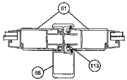
HEAVY DUTY ASTRAGAL HEAVY DUTY STILES
