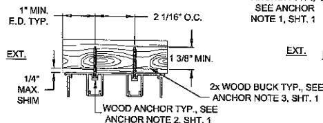
DETAIL B, 2-TRACK FRAME HEAD WOOD INSTALLATION
