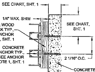
DETAIL D, 2-TRACK FRAME JAMB CONCRETE INSTALLATION
