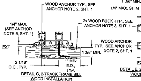
DETAIL C, 2-TRACK FRAME SILL WOOD INSTALLATION
