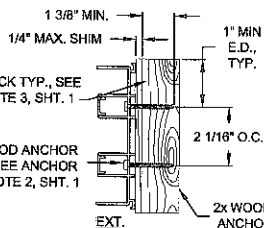
DETAIL E, 2-TRACK FRAME JAMB WOOD INSTALLATION
