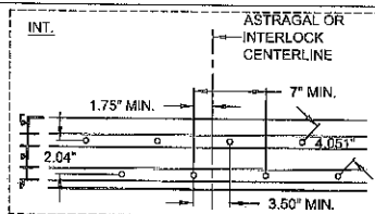
2-TRACK ASTRAGAL / INTERLOCK 8 ANCHOR CLUSTER
